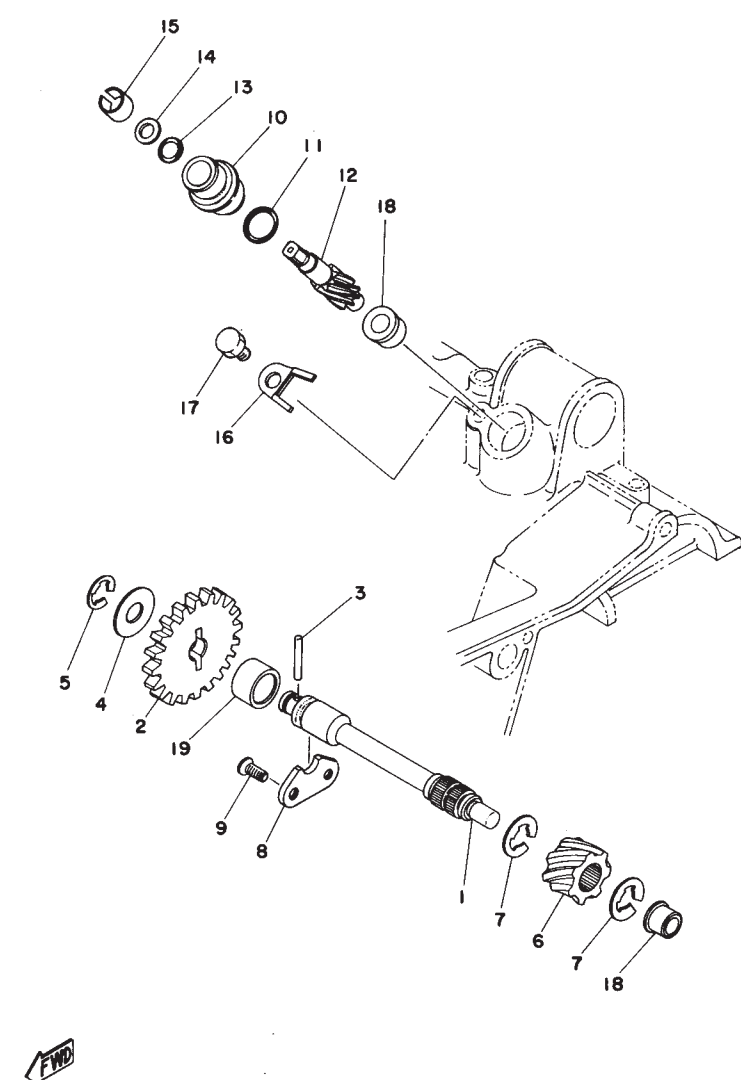
Fig. 10 TACHOMETER GEAR
