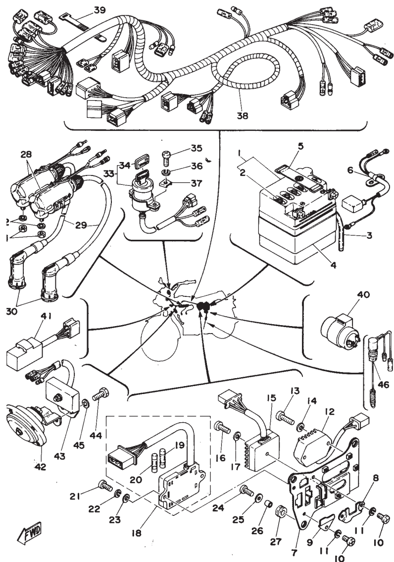
Fig. 46 ELECTRICAL
