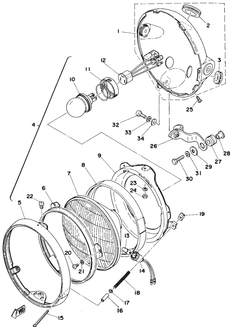
Fig. 41 HEAD LAMP 3
