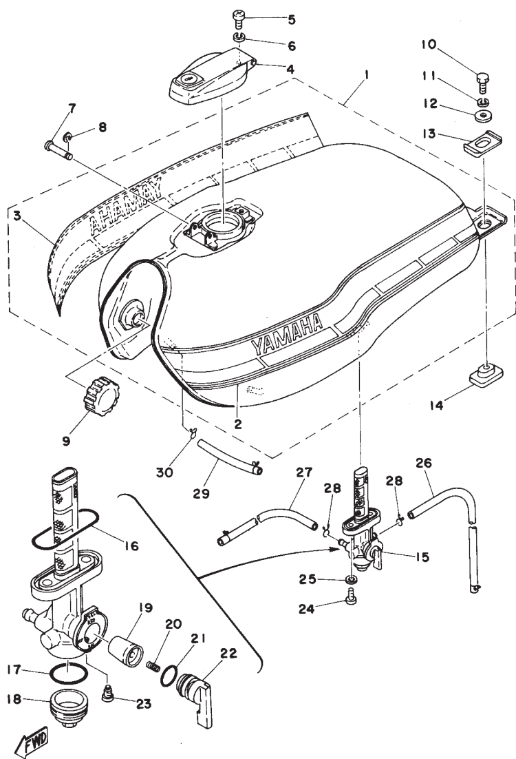
Fig. 27 FUEL TANK
