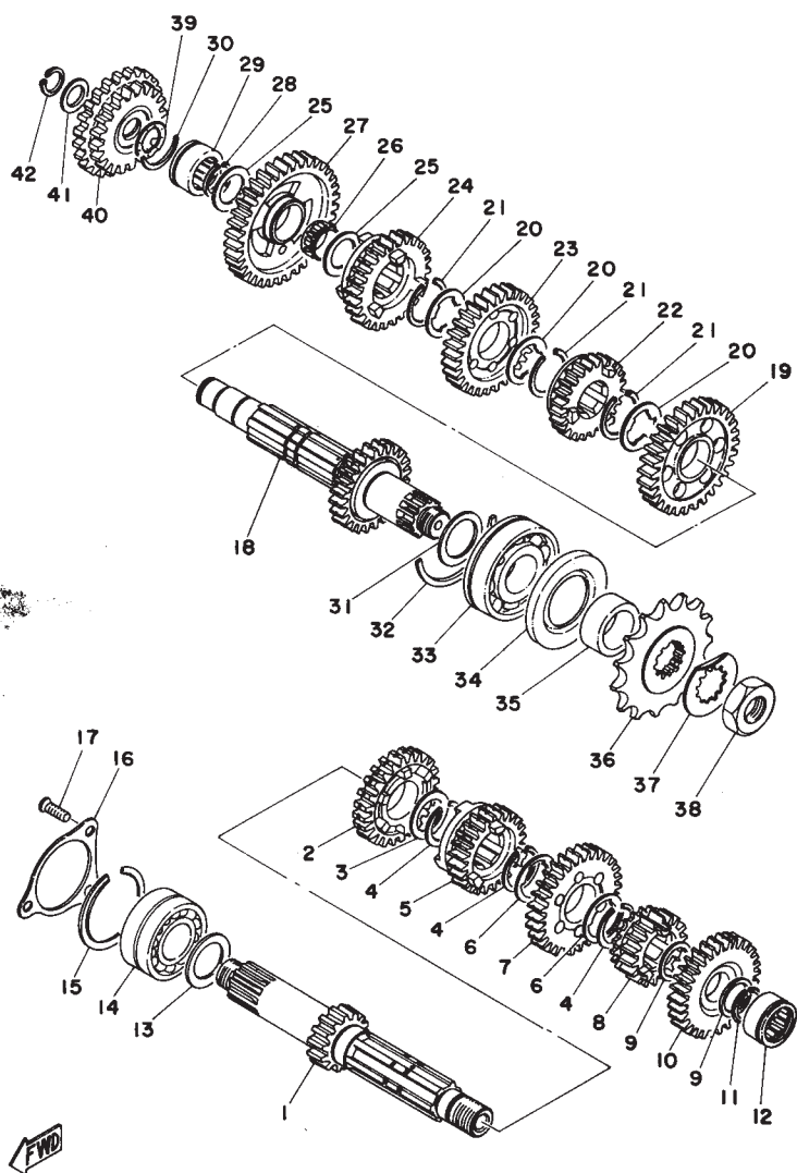
Fig. 6 TRANSMISSION
