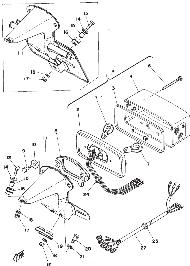
Fig. 43 TAIL LAMP
