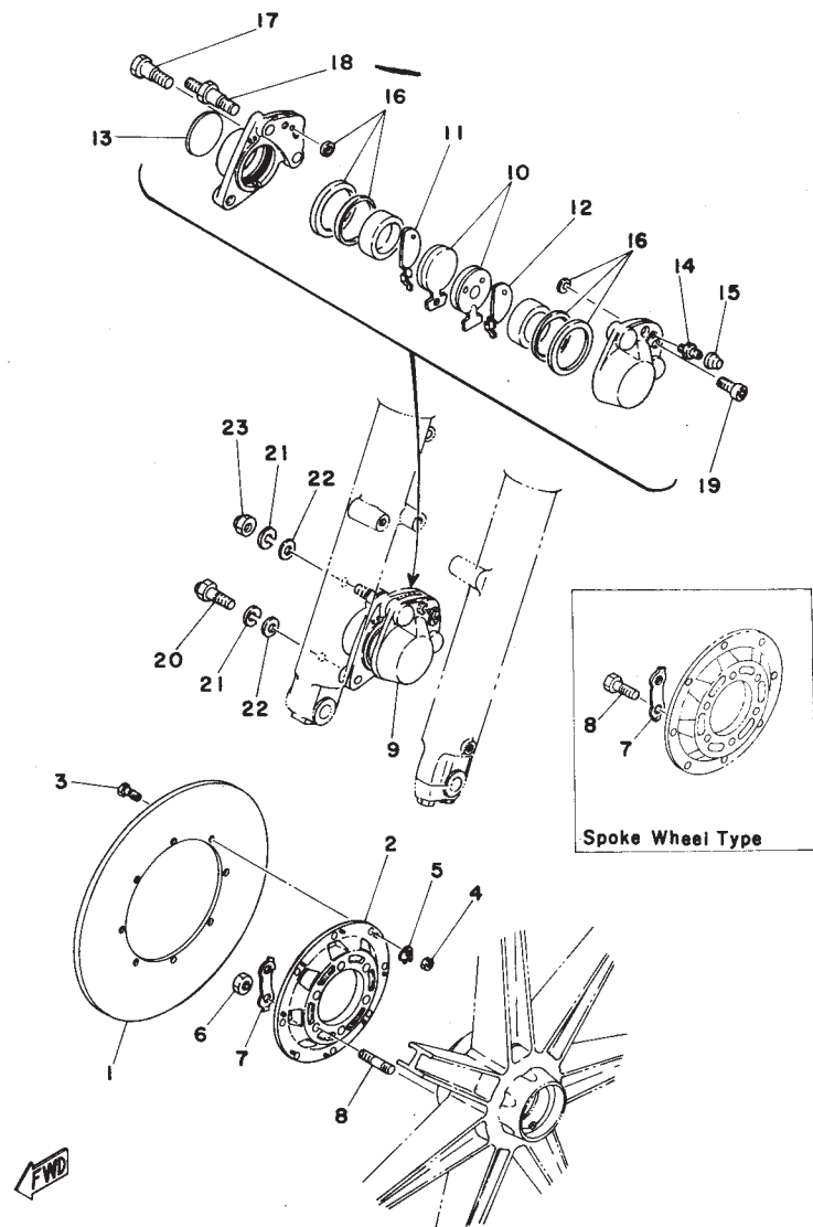
Fig. 33 FRONT DISK BRAKE · CALIPER
