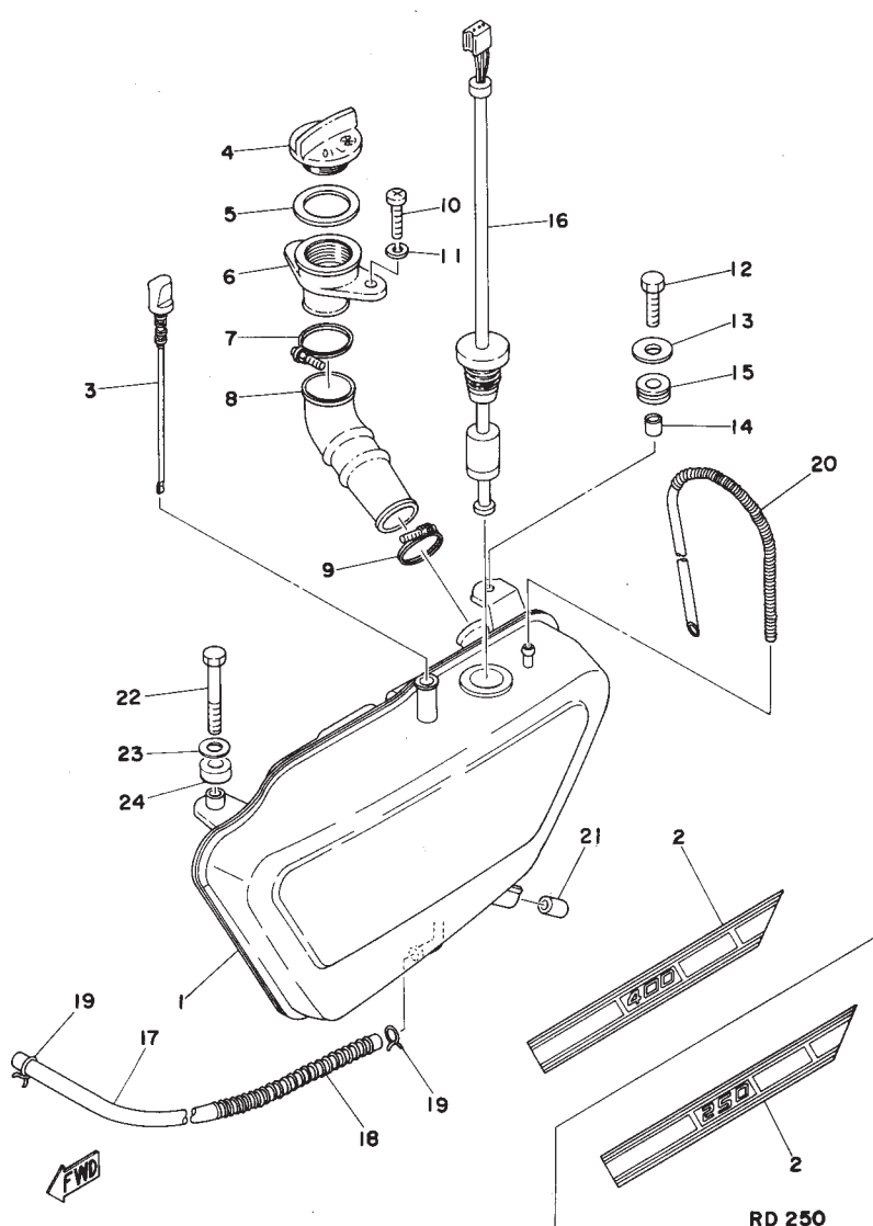
Fig. 28 OIL TANK
