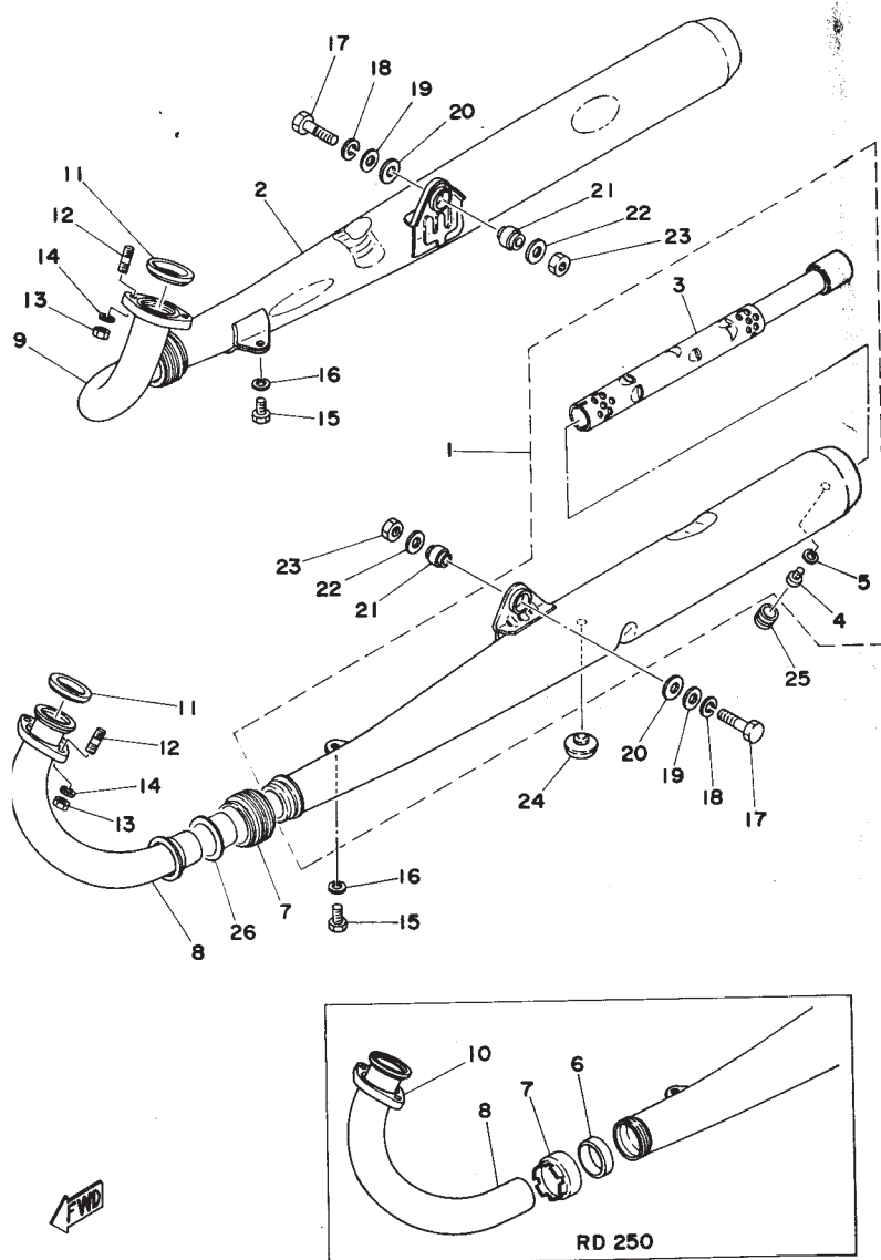
Fig. 13 EXHAUST
