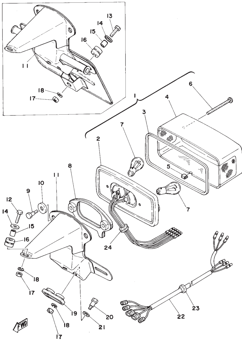
Fig.43 TAIL LAMP
