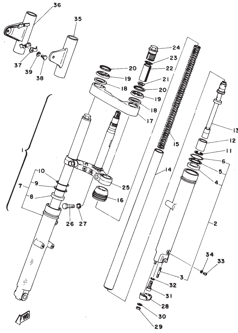
Fig. 23 FRONT FORK
