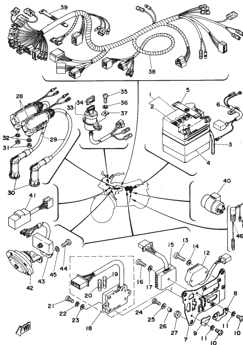
Fig. 46 ELECTRICAL
