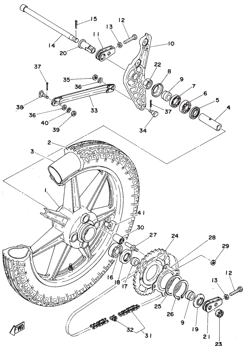
Fig. 36 REAR WHEEL (RD400: Casting Wheel Type)
