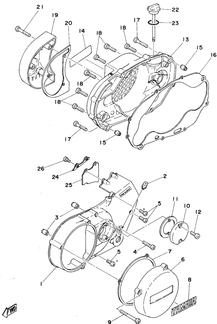
Fig. 3 CRANKCASE COVER
