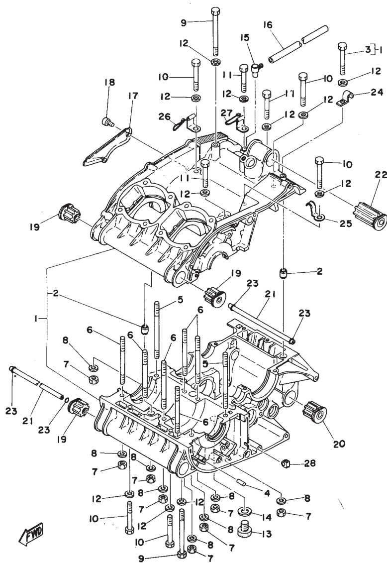
Fig. 2 CRANKCASE
