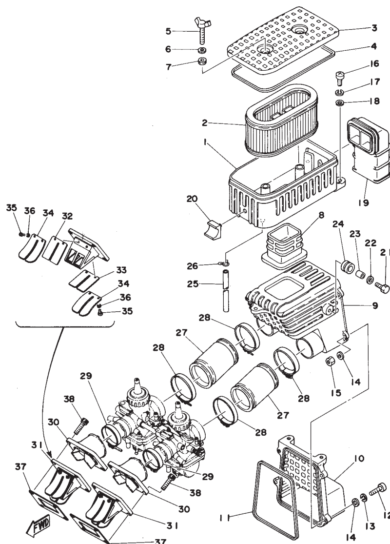
Fig. 11 INTAKE
