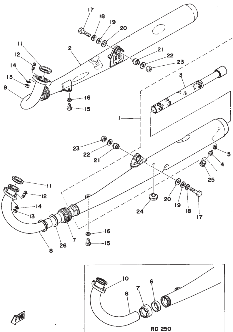
Fig.13 EXHAUST
