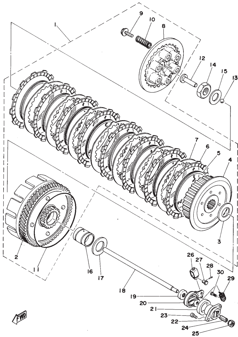
Fig.5 CLUTCH
