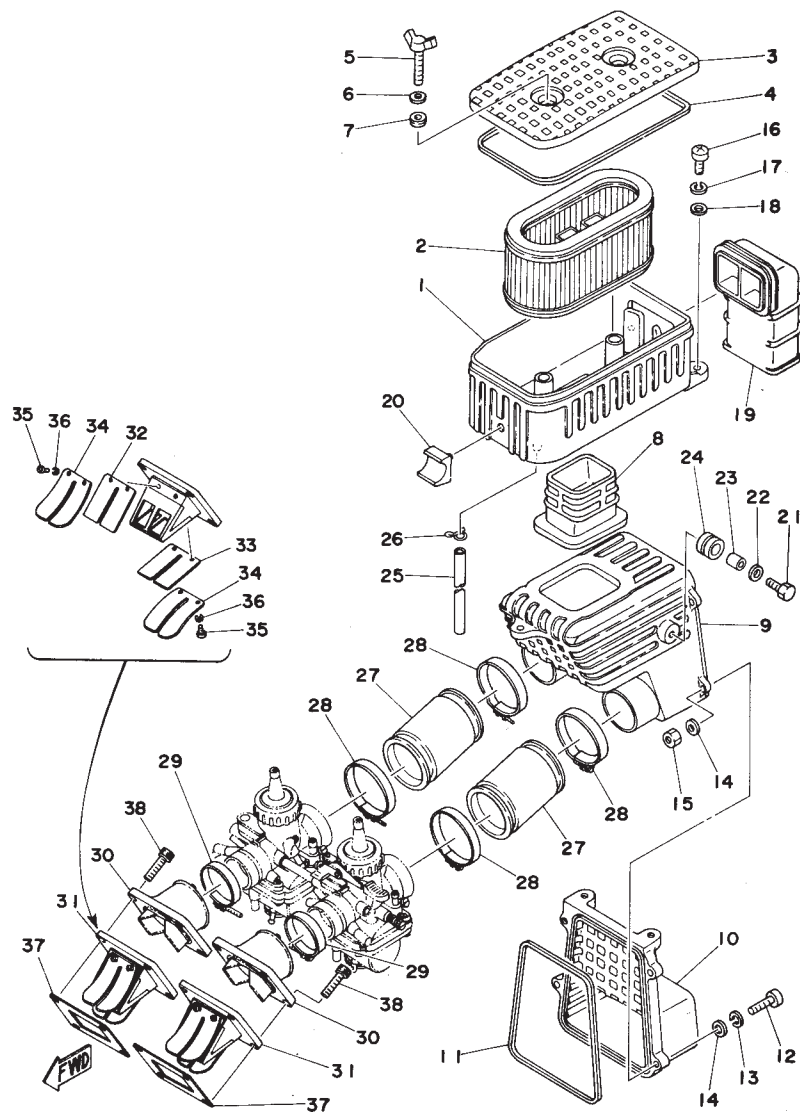
Fig. 11 INTAKE
