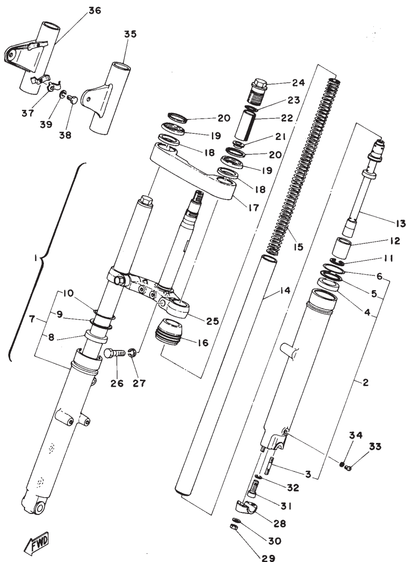
Fig. 23 FRONT FORK
